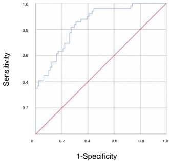
ROC curve
